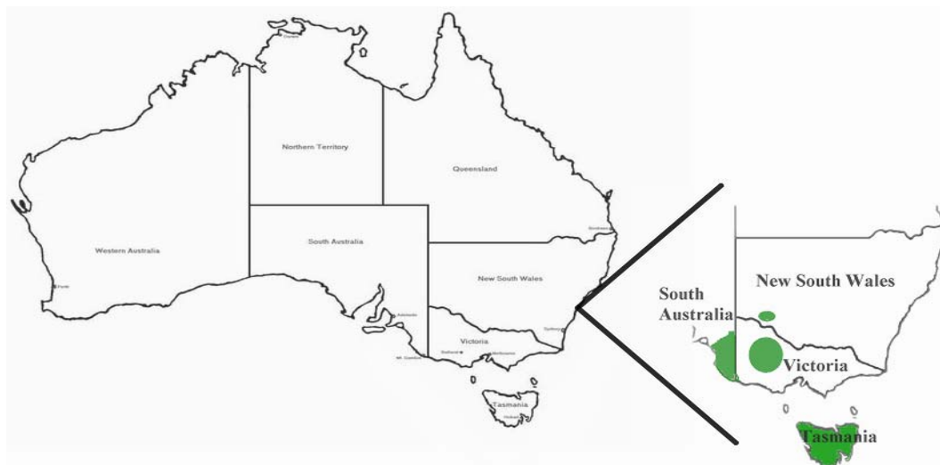
Fig 2.1. Map of Australia showing the location of sampling sites during the surveys from 2001 to 2004.
