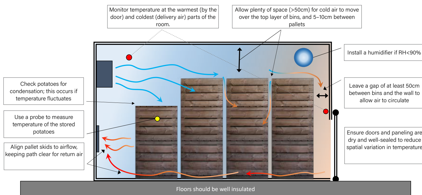
Figure 2. Cold storage rooms should be set up to allow the cold air to circulate around the bins; leave gaps between pallet stacks and the walls, align pallet skids to airflow; leave clear space for the return air intake. Temperature should be monitored and condensation checked in different parts of the room as well as in the stored seed (Source: J. Ekman)
