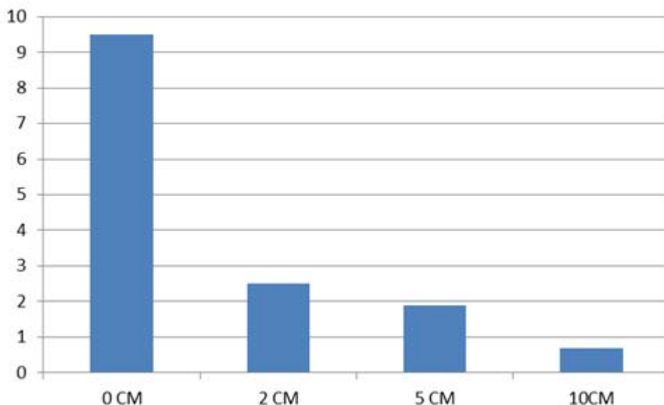
Figure 28. Development of stable flies from crop residues buried in the field at 2, 5 and 10cm without any compaction when stable fly numbers were low (October, 2015)
