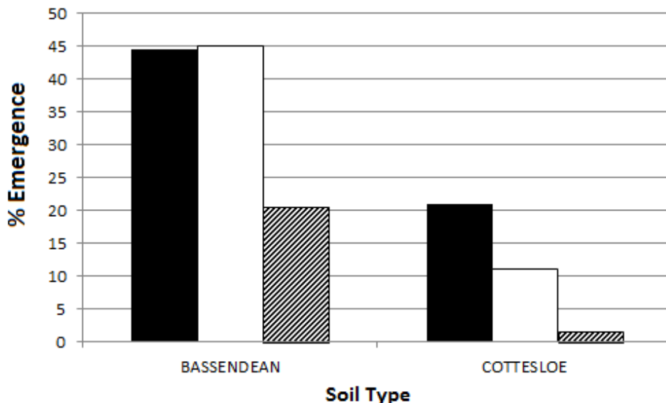
Figure 34. % stable fly emergence from pupae buried under moist Bassendeau or Cottesloe sandy soil either left non-compacted (Solid), compacted at either 3t/m 2 (Clear) or 5t/m 2 (Striped)
