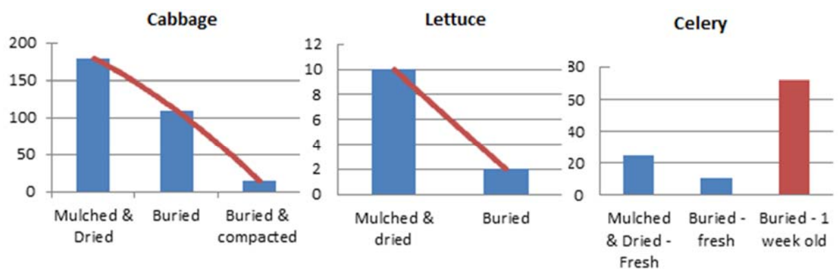
Figure 22. Field Trials on the impact of burial and compaction on cabbage residues, burial of lettuce residues, and burial of fresh v 1 week old celery residues on stable fly development. The y-axis is numbers of stable fly/m 2
