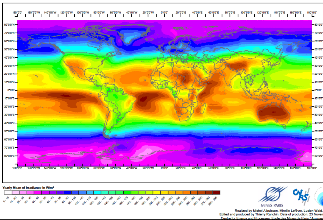
Figure 2. Global annual solar radiation levels (w/m 2 ).
